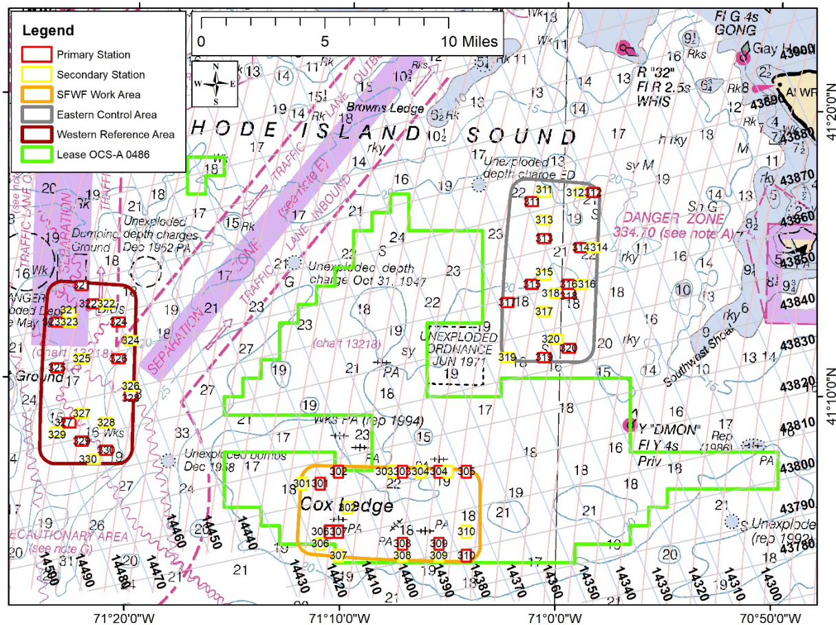
Figure 1. The South Fork Wind Farm (SFWF) development area and two reference control areas monitored by the ventless trap survey. Primary stations were sampled in all three areas;
